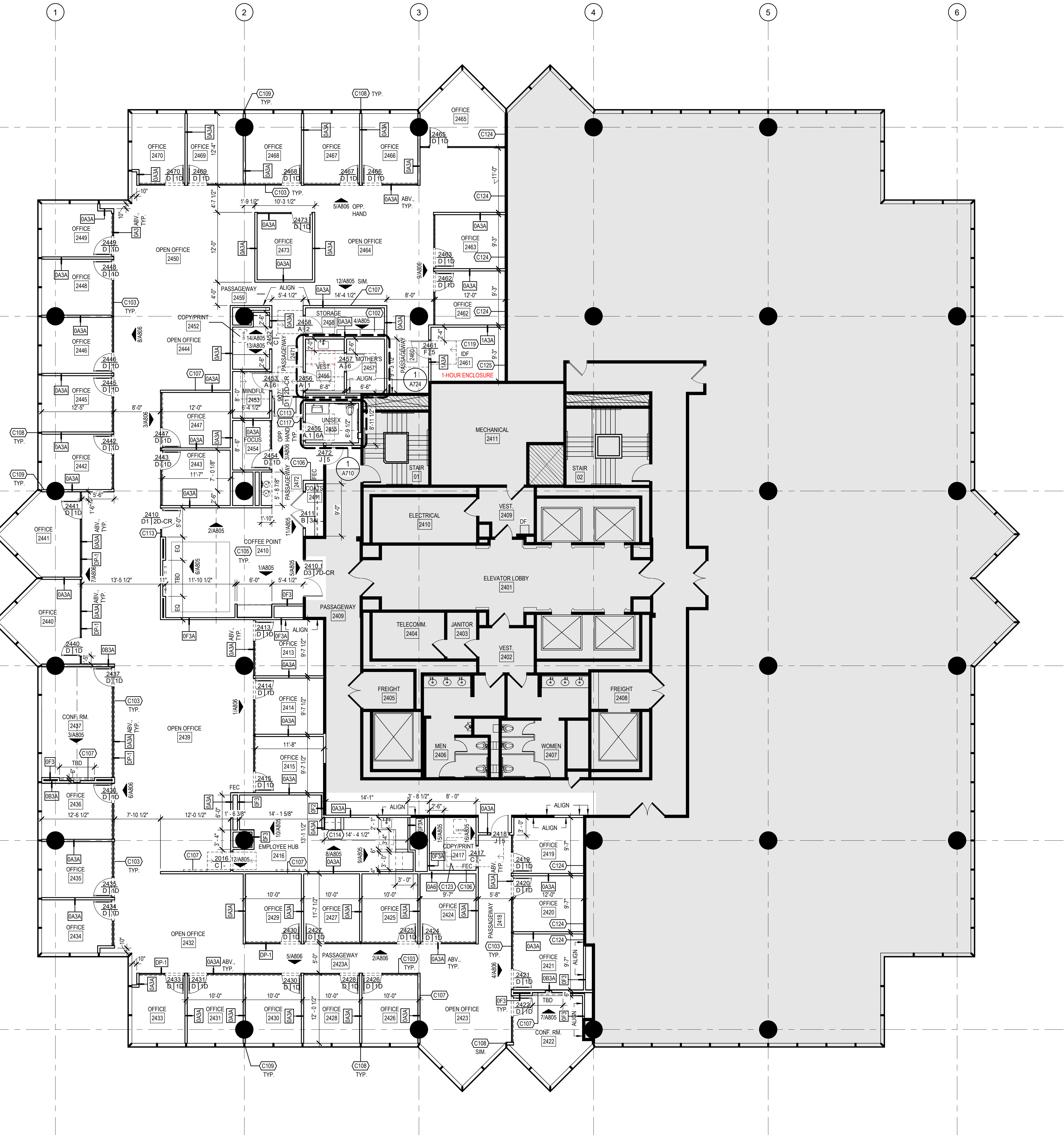
1 FLOOR PLAN - LEVEL 24 1/8" = 1'-0"
